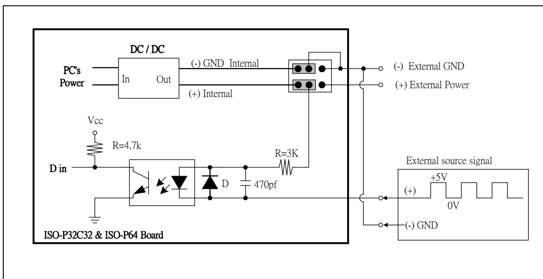
Figure 2-6. Typical Applications of D/I with internal power supply.
