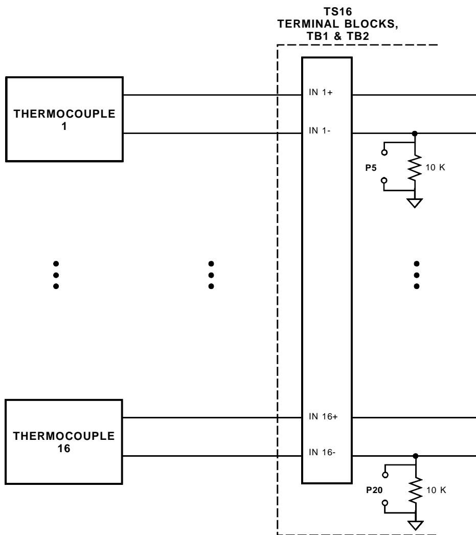
Fig. 2-3 — Thermocouple Connections
