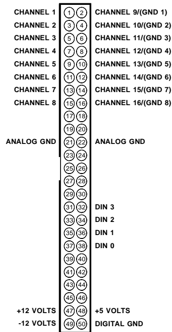
Fig. 2-1 — P1 I/O Connector Pin Assignments
