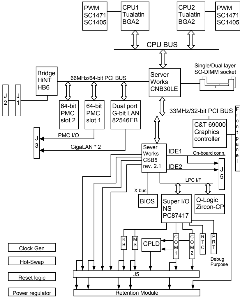
Figure 1. cPCI-6810/6820 Block Diagram
