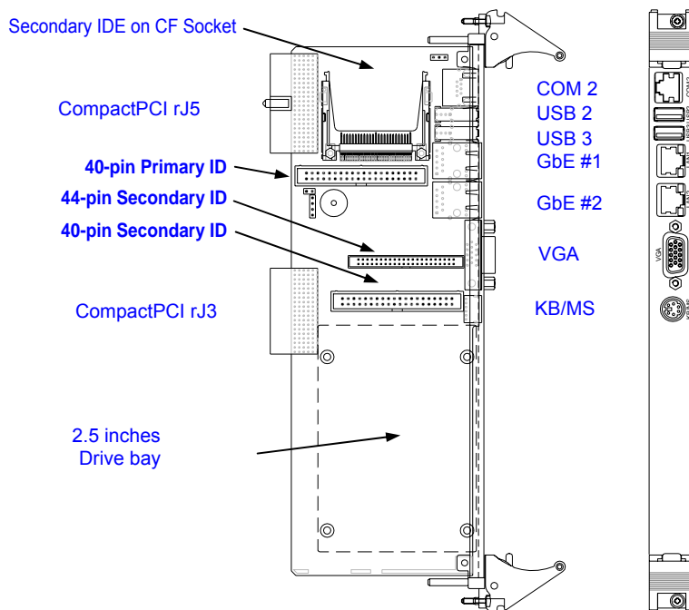
Figure 4. Top and front View of cPCI-R6820
