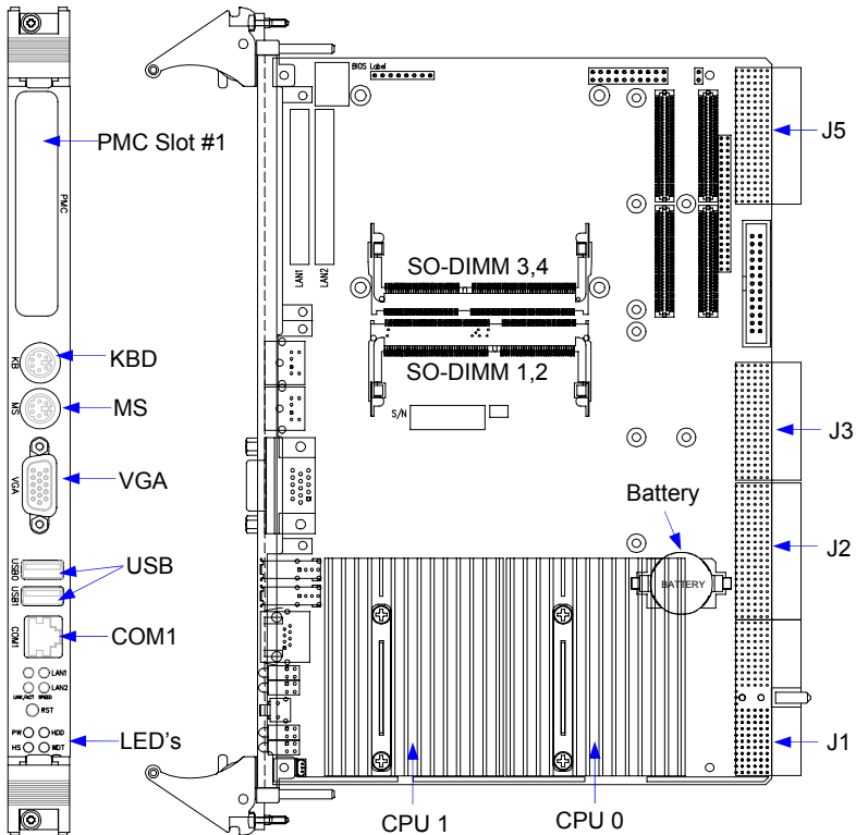
Figure 2. Top and Front View of cPCI-6820
