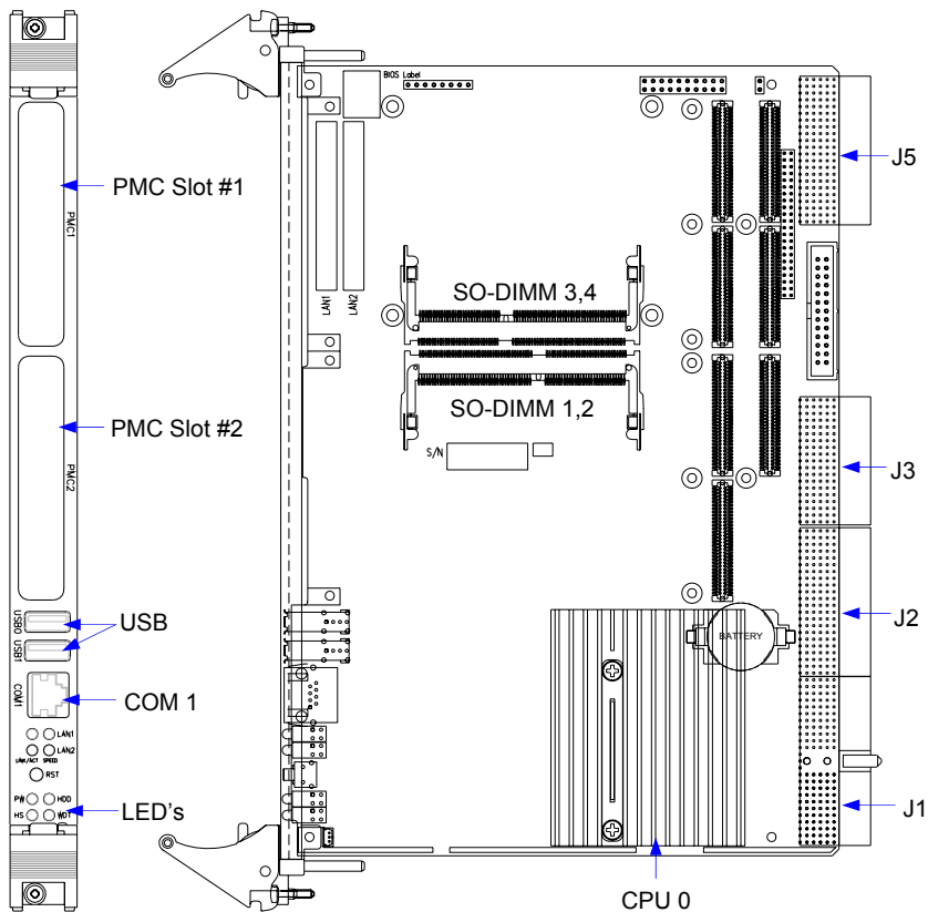
Figure 3. Top and Front View of cPCI-6810
