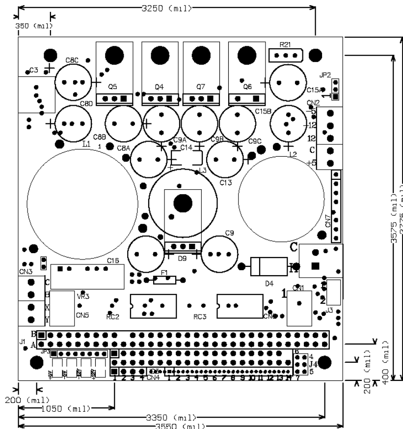
Figure 1-1, HE104 Dimensions 1000mil = 1 inch
