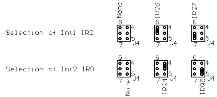
Figure 2-2, Interrupt IRQ Selection
