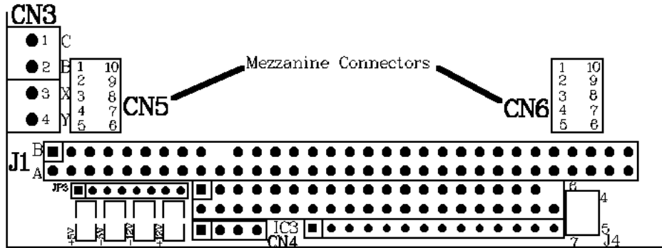
Figure 2.3, HE104 Mezzanine Connectors
