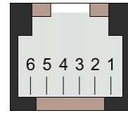
RJ12 6Pin Female
