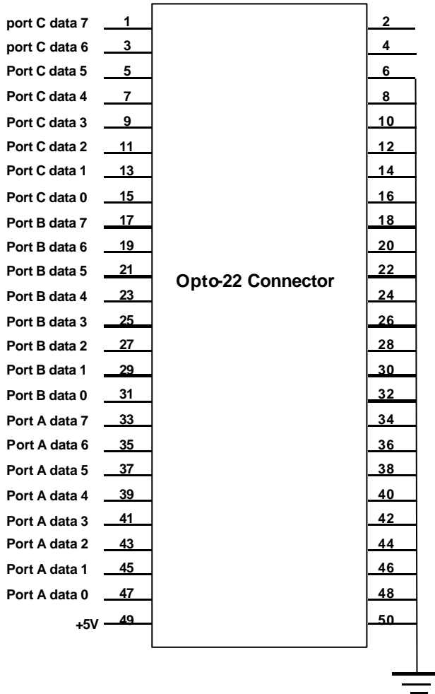
CN5 pin definition
