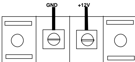
CN5 Connection
