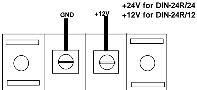
CN5 connection
