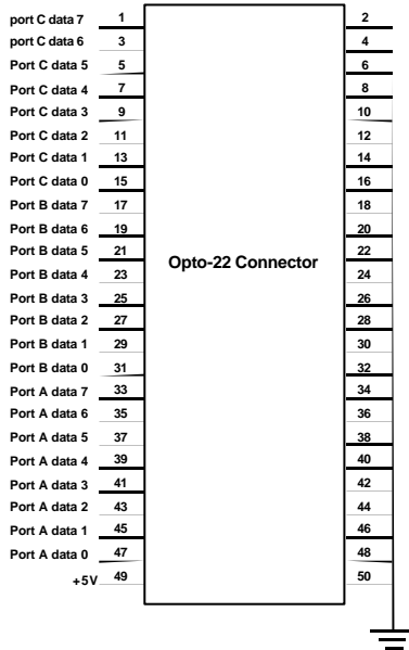
CN6 pins define figure
