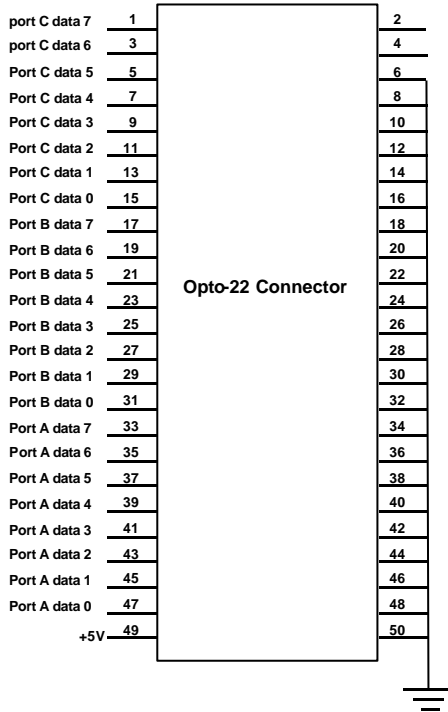
CN6 pin definition
