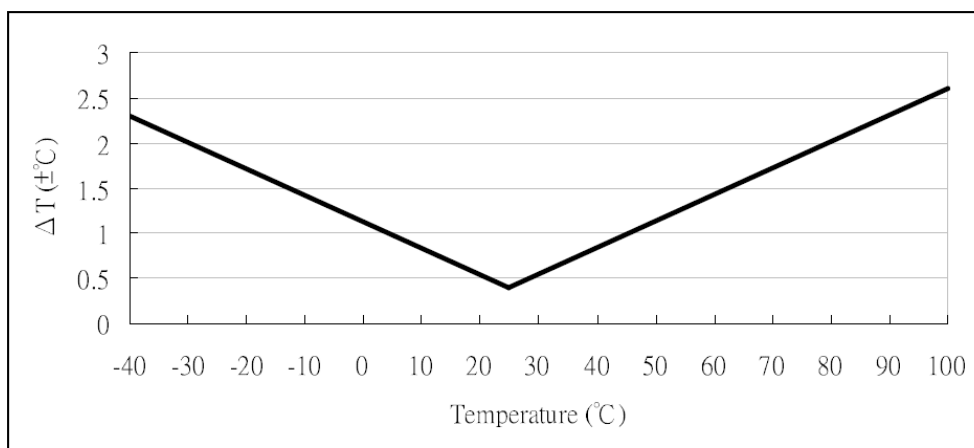
Figure 2: Maximum T-tolerance per sensor
