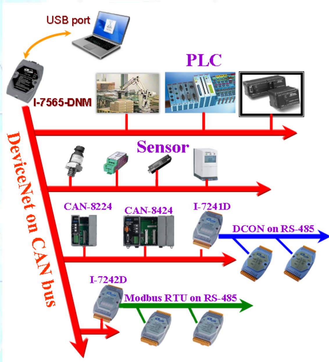
Figure 1.3 Application architecture
