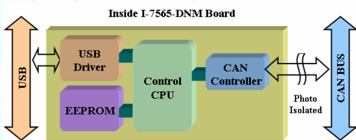
Figure 1.8 Block diagram of the I-7565-DNM
