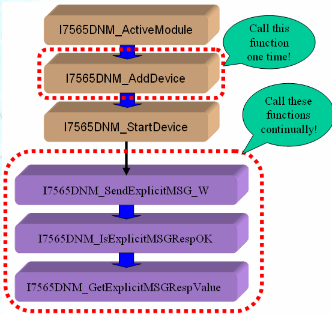
Figure 3.9 “SendExplicitMSG_W” Diagram
