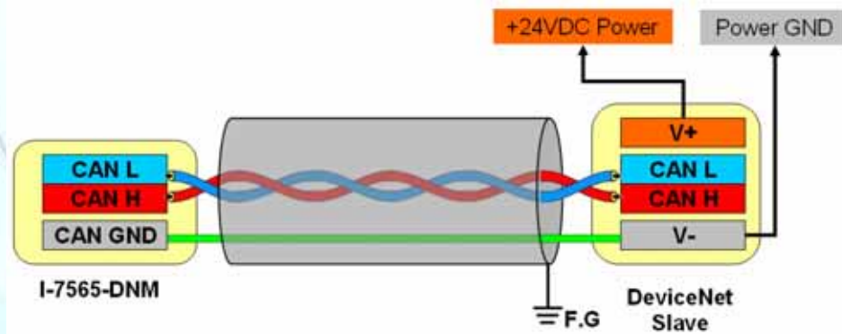
Figure 2.6 CAN bus wire connection with 24VDC power
