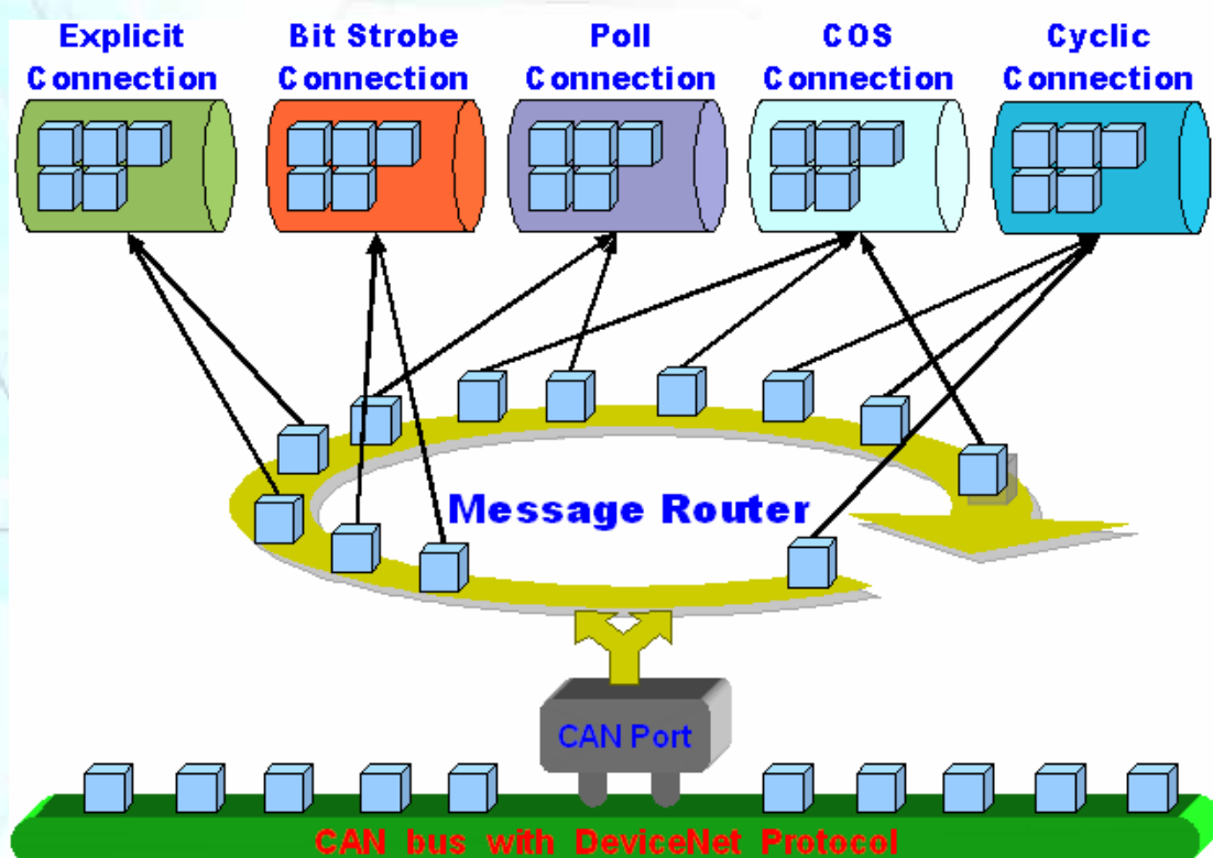
Figure 1.6 Message Router
