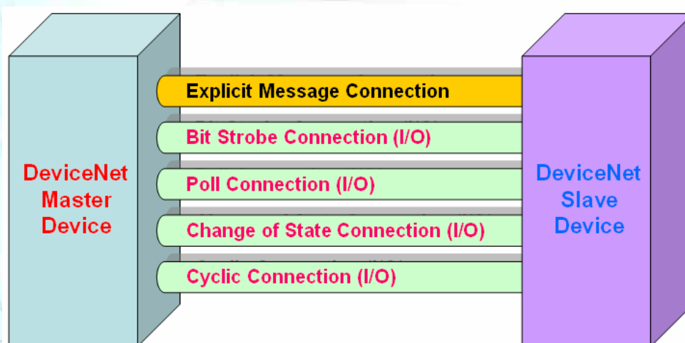
Figure 1.4 DeviceNet Messaging
